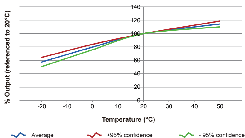
Temperature Performance of SemeaTech Commercial CO-1000 Sensor
