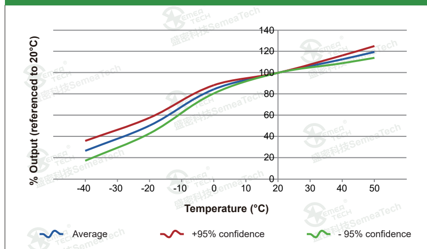
Temperature Performance of SemeaTech Commercial CO-1000C Sensor
