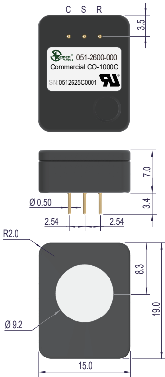
All dimensions in mm All tolerances \pm 0.20 mm unless otherwise stated
